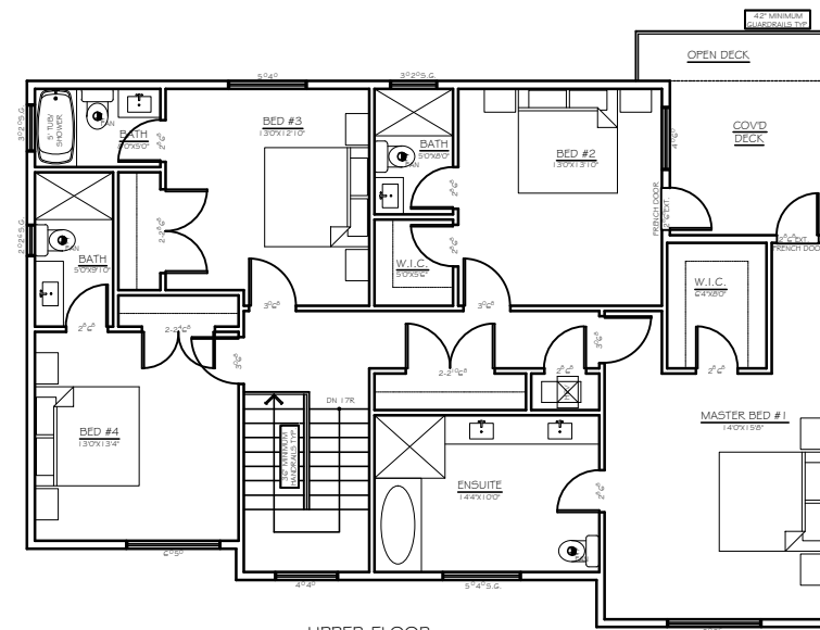
UPPER FLOOR SCALE: 1/4" = 1"
